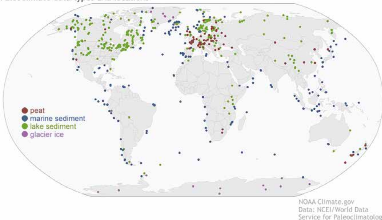
Paleoclimate data types and locations
