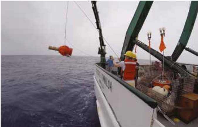
A deep Sounding Oceanographic Lagrangian Observer (SOLO) float deployment off the R/V Ka'imikai-O-Kanaloa during a Hawai'i Ocean Timeseries (HOT) cruise in the Pacific. Photo credit: Blake Watkins, University of Hawai'i (May 2019)
