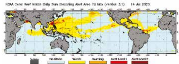
NOAA Coral Reef Watch's daily global 5km satellite coral Bleaching Alert Area (7-day maximum) product for July 14, 2020. The Bleaching Alert Area (7-day maximum) is a composite product that outlines the current locations, coverage, and potential risk level of coral bleaching heat stress around the world. Data and images are produced globally at 5km-resolution and are updated daily. Photo credit: NOAA NESDIS/Coral Reef Watch.
